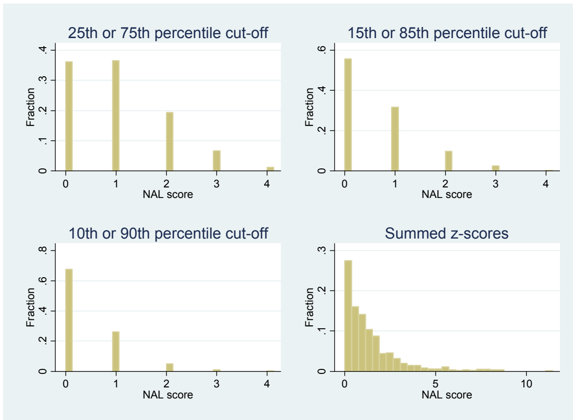
Figure 2 Distributions of neuroendocrine allostatic load (NAL) scores using various scoring methods
