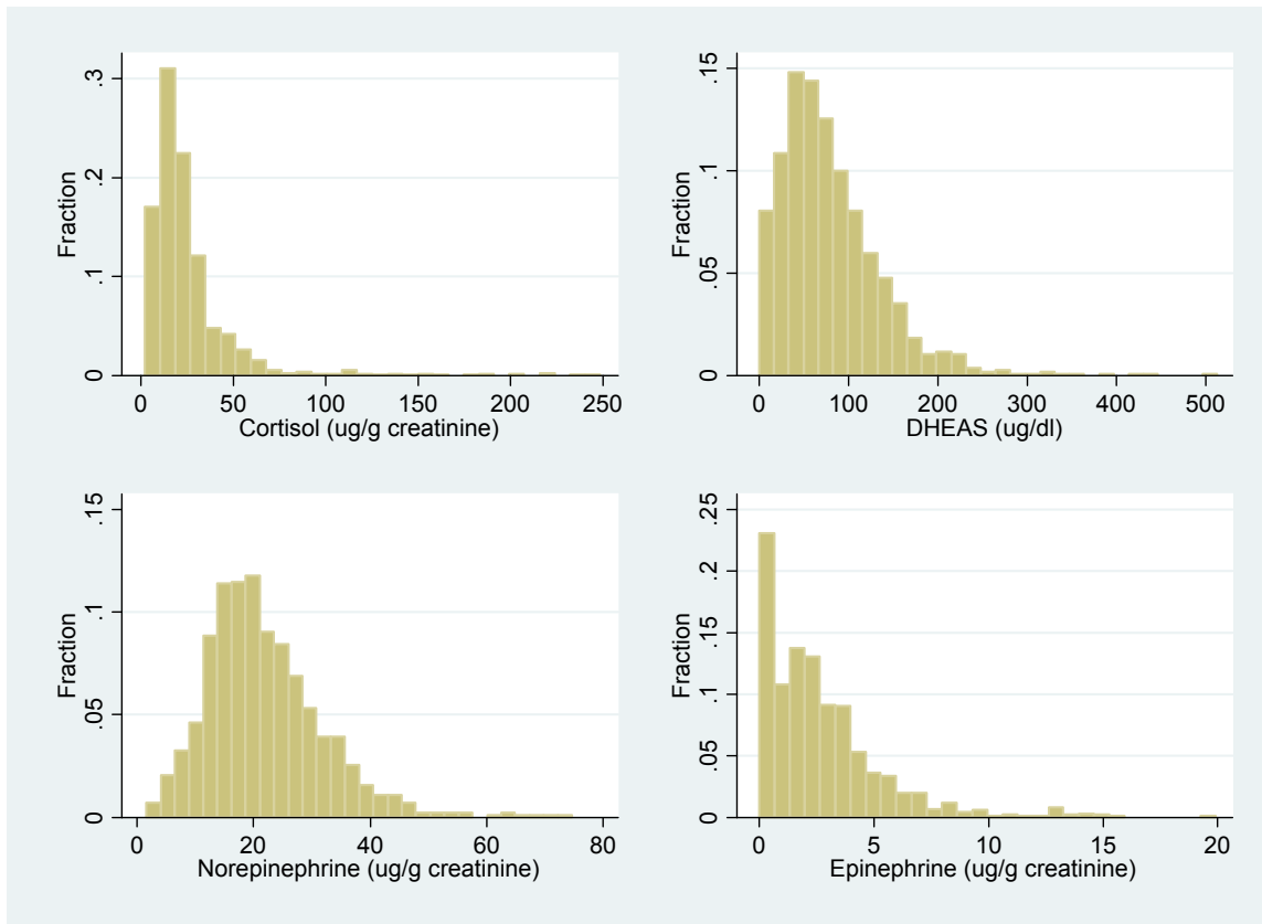
Figure 1 Histograms of the four neuroendocrine biomarkers
